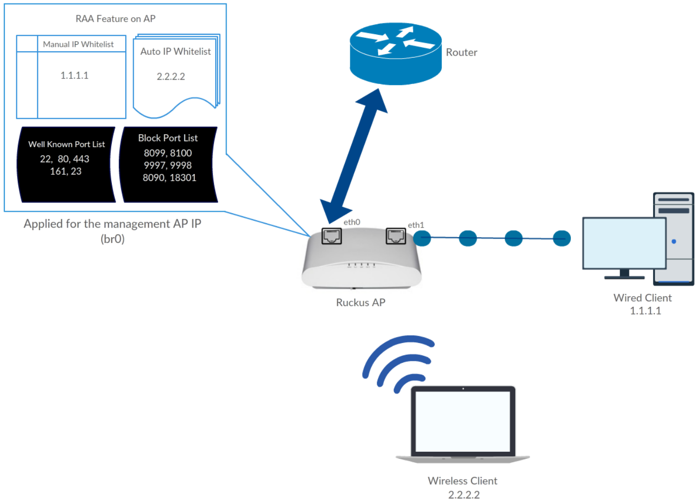
FIGURE 200 Restricted Access Overview
