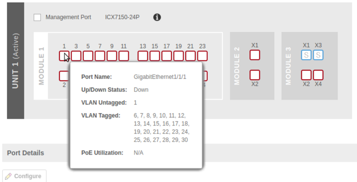
FIGURE 113 Front Panel View
