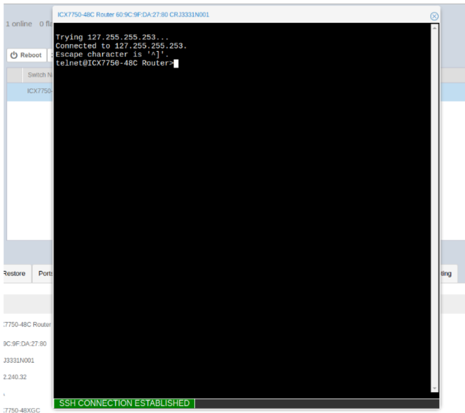
FIGURE 130 Accessing Switch Through the CLI Sesion
