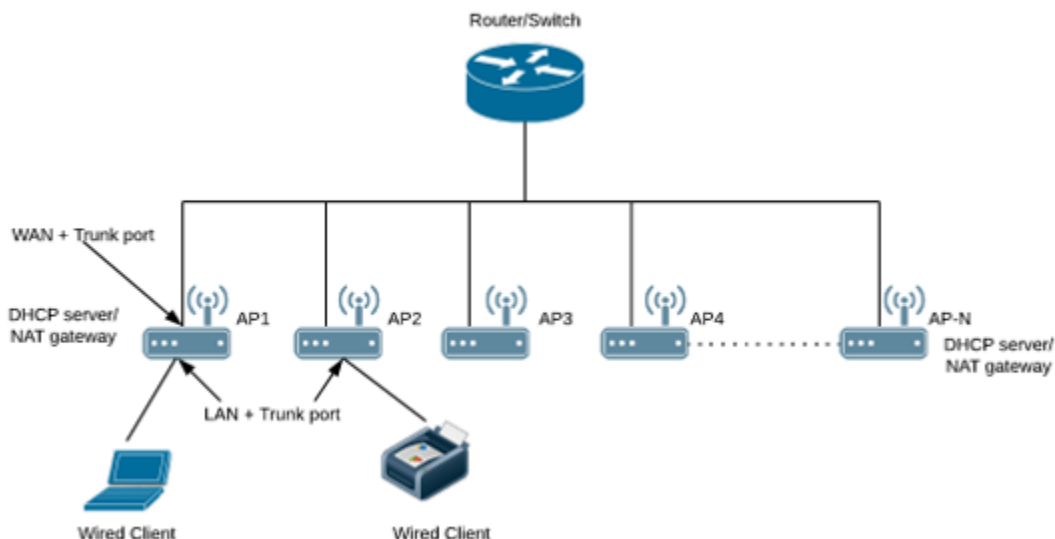
FIGURE 233 Single AP Topology
