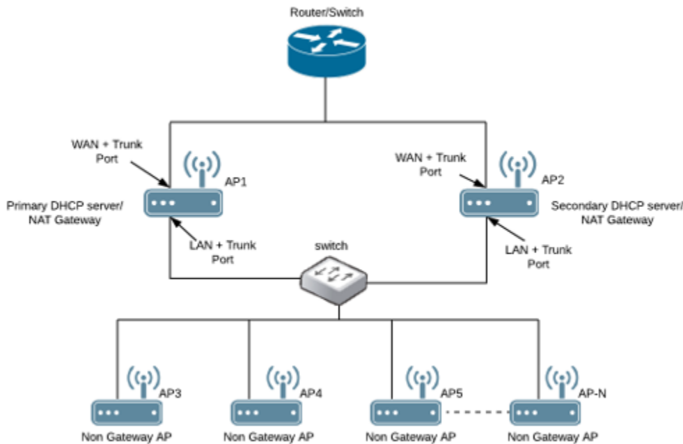
FIGURE 235 Hierarchical AP Topology
