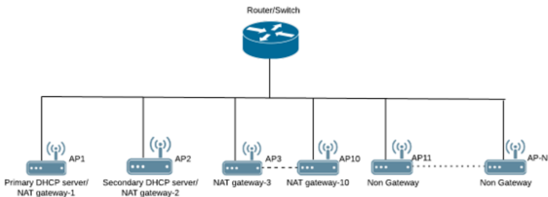
FIGURE 234 Multiple AP (Flat Network) Topology
